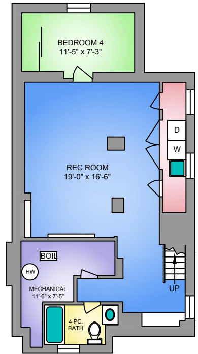
LOWER FLOOR 882 SQ. FT. 6'-2" CEILING
