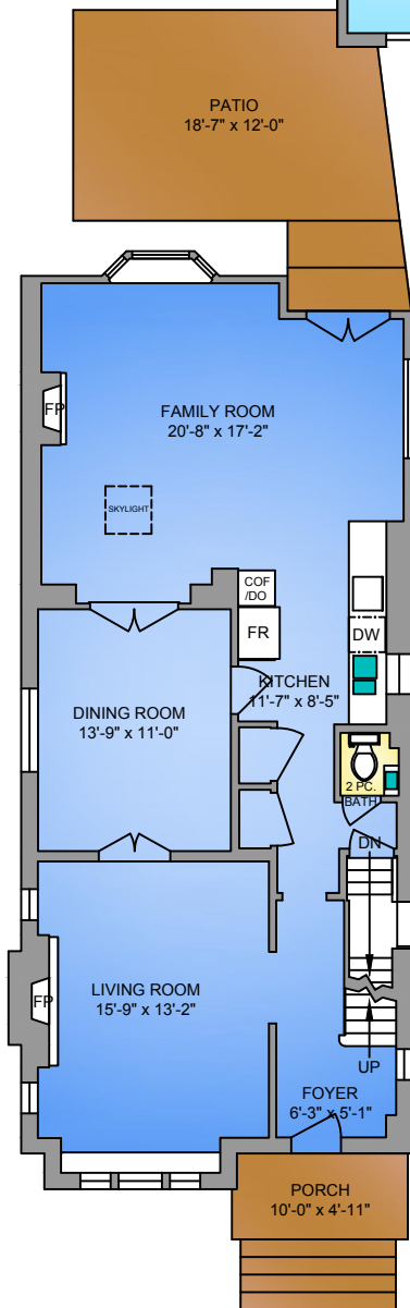
MAIN FLOOR 1133 SQ. FT. 8'-3" CEILING
