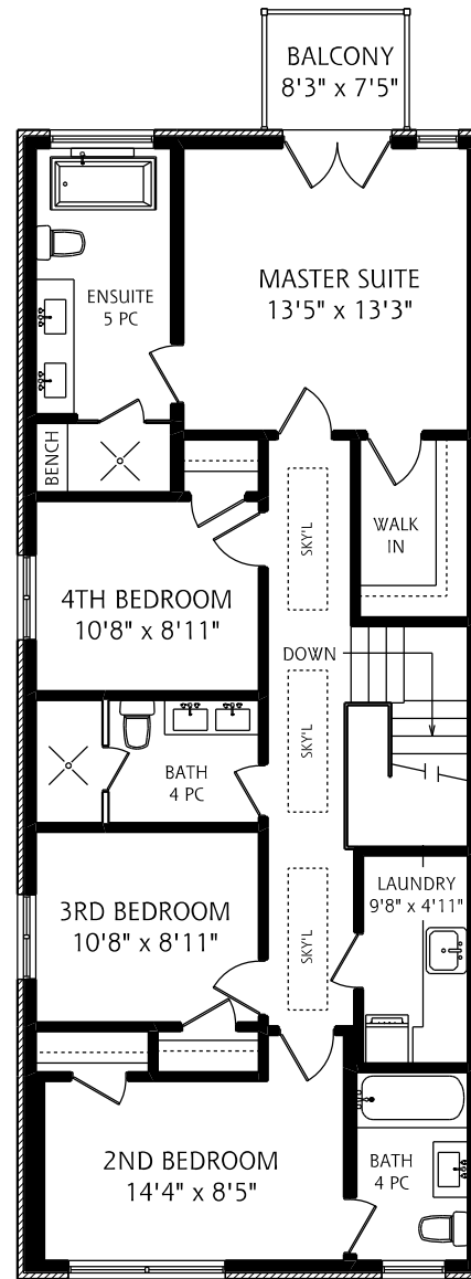
SECOND FLOOR 1,200 SQUARE FEET
