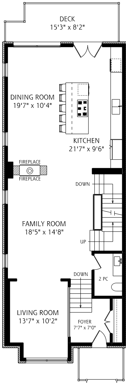
MAIN FLOOR 1,230 SQUARE FEET
